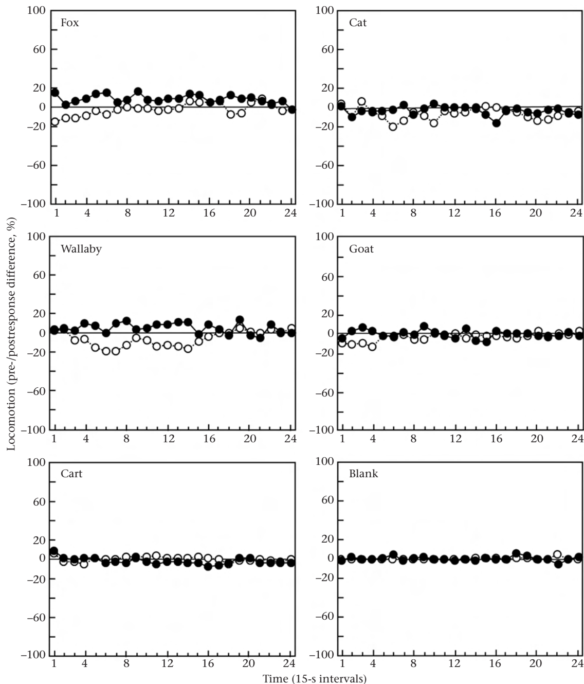
Figure 5. Changes in locomotion after training for the paired-experimental (●, N=8 ) and unpaired-control (○, N=8 ) groups. Mean differences have been calculated in the same way as for Fig. 3.
