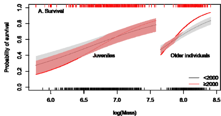
Figure S4. The relationship between body mass and survival for <2000 and ≥2000 years. Shaded areas indicate the 95% confidence intervals, and rugs above and below the graph represent the distribution of the body mass data.
