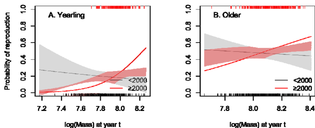
Figure S6. The relationship between body mass and age-specific probability of reproduction for <2000 and ≥2000 years. Shaded areas indicate the 95% confidence intervals, and rugs above and below the graph represent the distribution of the body mass data.
