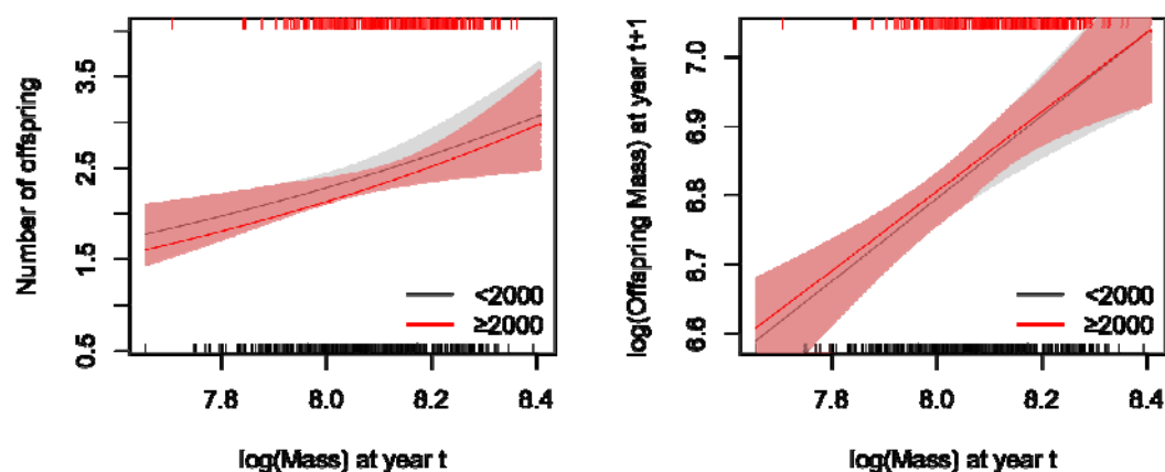
Figure S7. The relationship between body mass and (A) number of offspring produced and (B) offspring mass for <2000 and ≥2000 years. Shaded areas indicate the 95% confidence intervals, and rugs above and below the graph represent the distribution of the body mass data.
