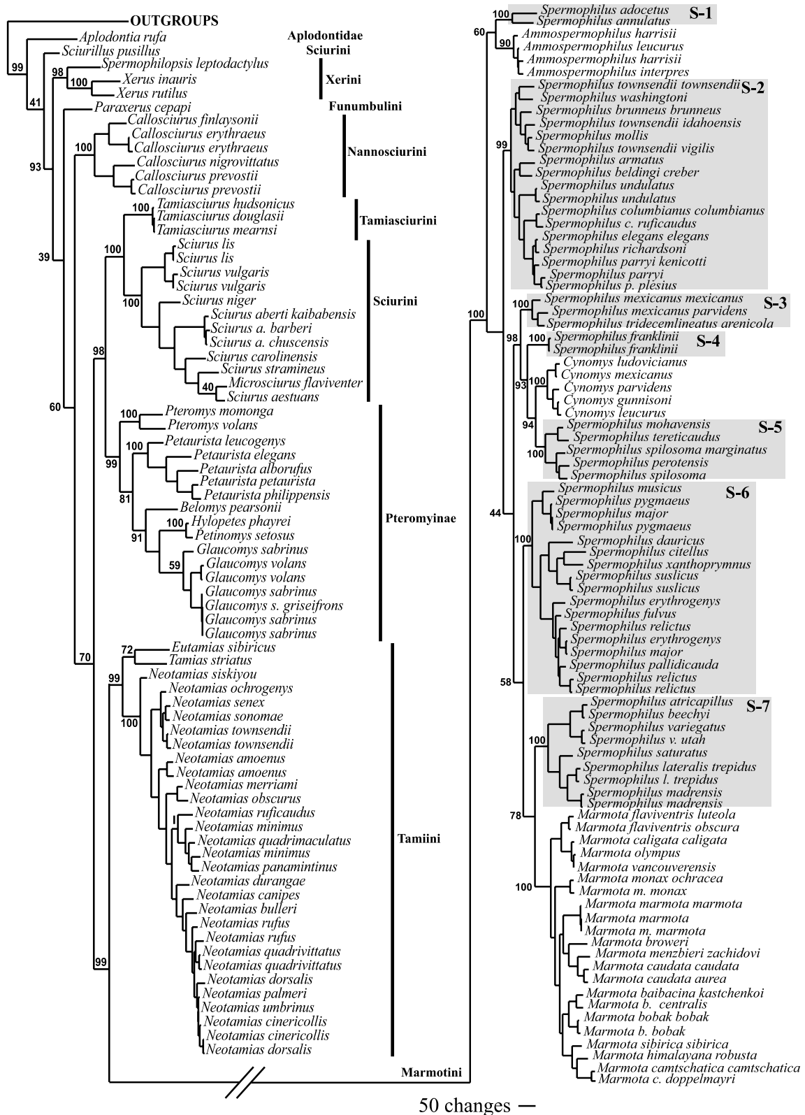
Fig. 3. Majority rule consensus phylogram (with branch lengths averaged over all trees) resulting from Bayesian phylogenetic analysis using a GTR + G + I model of evolution. Posterior probabilities estimated from a total of 4 million post-burn-in generations (from four independent runs) are indicated for major nodes. Higher taxon names are also given. Seven clades representing independent lineages containing members of the genus Spermophilus are indicated by sequentially labeled shading (S-1 to S-7).
