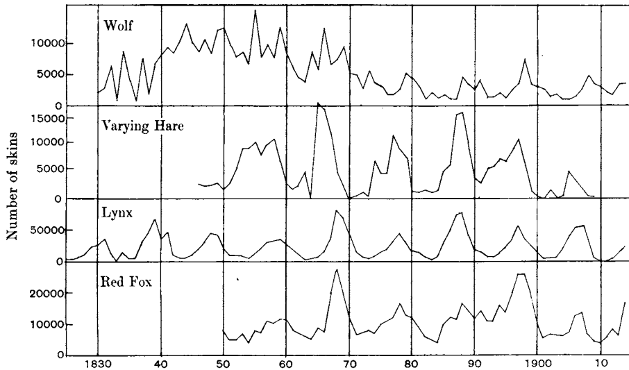
Fig. 2. Fluctuations in the numbers of Canadian mammals (from Hewitt, 1921). The figures for any one year represent wholly or partly the effect of numbers in the summer of the year before. In the case of the lynx there may be a lag of more than one year, on account of various trapping factors.
