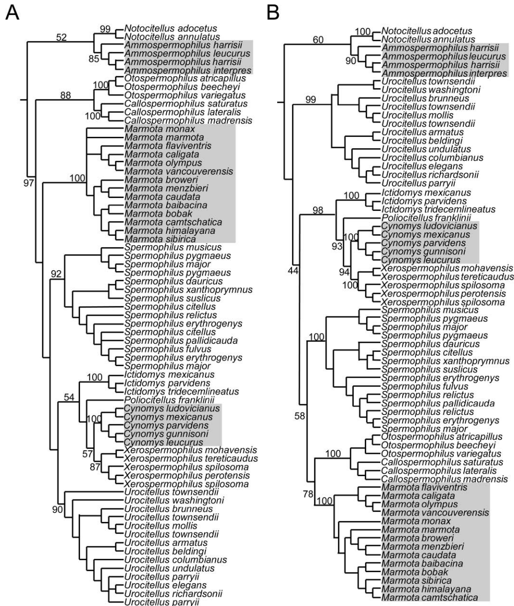
FIG. 2. —Phylogeny of Marmotini proposed by Herron et al. (2004) based on analyses of complete sequences of the cytochrome- b gene. Harrison et al. (2003) presented very similar results. Multiple terminal branches representing the same taxon have been collapsed for simplification in some cases, and some identifications have since been modified. The shaded taxa represent the 3 genera that have not been traditionally recognized in Spermophilus . A) Maximum parsimony: “Strict consensus of all 208 equally optimal trees based on unweighted maximum parsimony search” (Herron et al. 2004:1022). Bootstrap percentages for nodes of taxonomic interest (generic and supergeneric) are shown following Herron et al. (2004). B) Bayesian analysis: “Majority rule consensus phylogram (with branch lengths averaged over all trees) resulting from Bayesian phylogenetic analysis using a GTR + G + I model of evolution” (Herron et al. 2004:1024). Posterior probabilities “estimated from a total of 4 million post-burn-in generations (from four independent runs)” are provided for nodes of taxonomic interest (generic and supergeneric) following Herron et al. (2004:1024).
