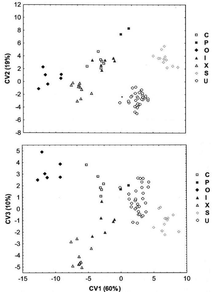
FIG. 5.—Discriminant function analysis highlighting craniometric distinctions between generic lineages within Marmotini, excluding the genera Marmota , Cynomys , Ammospermophilus , and Notocitellus (see Fig. 3). All lineages achieve discrimination along the first 2 canonical variate roots (CV1 is shown along the horizontal axis in both plots), reflecting consistent differences in craniodental shape, with the exception of Callospermophilus and Ictidomys , ecomorphologically similar but phylogenetically unrelated genera (Fig. 2) that segregate along the 3rd canonical variate primarily on the basis of slight differences in size and comparative robustness (Table 2).
